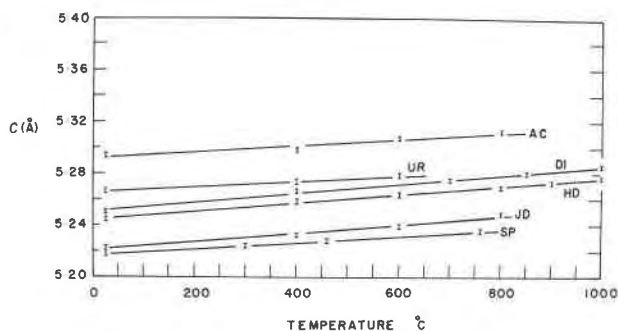
FIG. 4. Variation of c unit cell parameter with increasing temperature for six clinopyroxenes. (Abbreviations are the same as those in Figure 2.) Error bars represent \pm 1 standard deviation.
