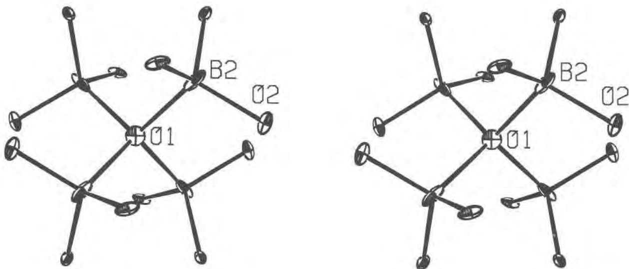
FIG. 3. Stereographic-pair view of the coordination around O(1) in the cubic structure, looking along a cubic axis. Thermal ellipsoids for 50 percent probability. Drawing produced by ORTEP (Johnson, 1965).
