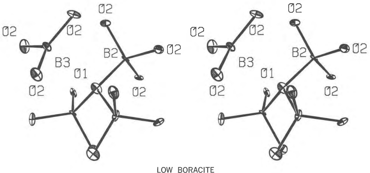
FIG. 1. Stereographic-pair view of the coordination around O(1) in the orthorhombic structure, looking approximately along b but rotated +30^\circ around c . The approach, B(3)-O(1), is 2.303 \text{ \AA} . Thermal ellipsoids are for 50 percent probability. Drawing produced by ORTEP (Johnson, 1965).
