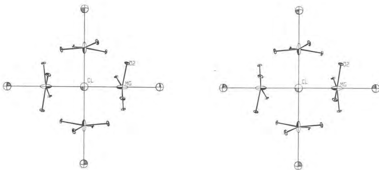
FIG. 2. Stereographic-pair view of the chlorine coordination looking along a cubic axis. Thermal ellipsoids for 50 percent probability. Drawing produced by ORTEP (Johnson, 1965).
