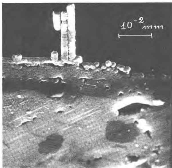
FIG. 5. Nearly smooth microcrystalline crust of goethite.
