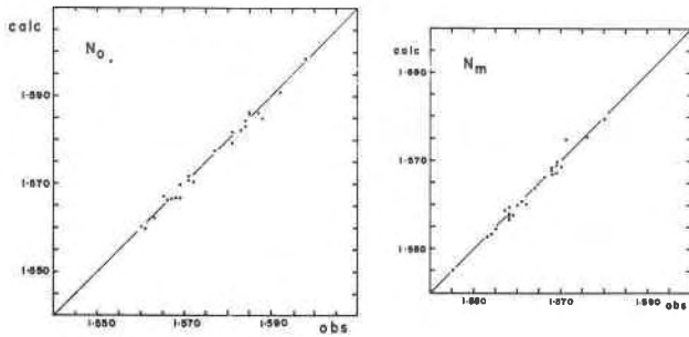
FIG. 3. Plots of refractive indices (observed vs. calculated). Calculated indices are estimated with equations 1–2, Table 4. The 45-degree line indicates perfect fit.
