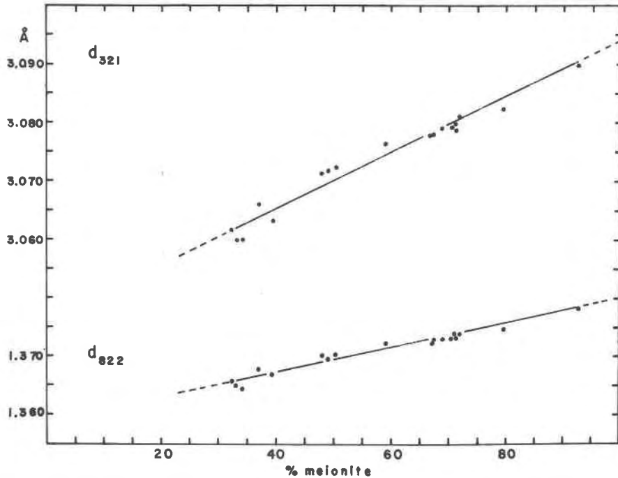
FIG. 6. Change of d -spacings with composition. Regression lines are those of equations 7–8, Table 4.
