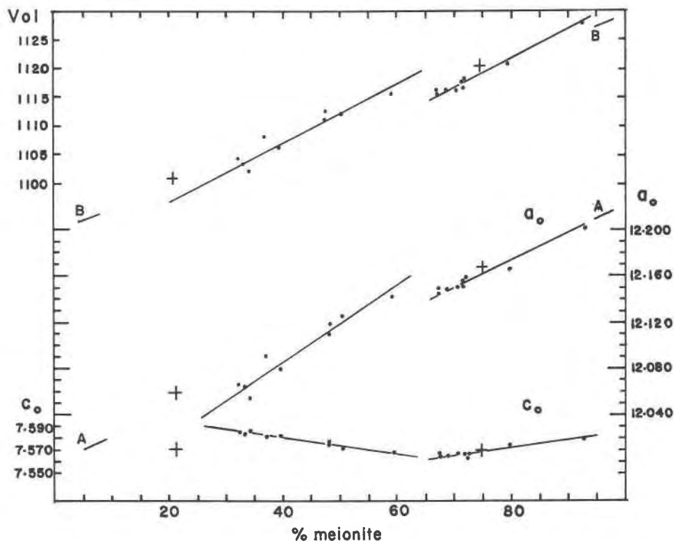
Fig. 1. Variation of cell parameters with meionite content. Cell edges in Angstroms, cell volume in cubic Angstroms. Dots indicate cell dimensions measured with Guinier camera; crosses are values from the literature (see Table 3). Traces AA and BB are plots of linear equations 3-4, Table 4, and may be used for estimating meionite content in specimens of unknown composition.
