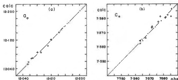
FIG. 5. Plots of cell edges (observed vs. calculated) in Angstroms. Calculated cell edges are from equations 4, 5, 10 and 11, Table 5. Crosses: compositions up to 66 percent meionite; dots: over 66 percent.
