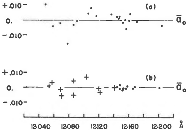
FIG. 4. Plots of residuals vs. a(\text{calc}) in Angstroms. a) Results for single-population model; b) Two populations with a "break" at about 66 percent meionite.
