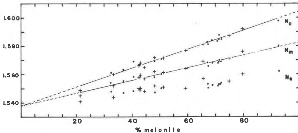
FIG. 2. Refractive indices of scapolites as a function of composition. Dots are measurements reported there, crosses are values taken from Shaw (1960a). n_o and n_e : indices of the ordinary and extraordinary rays. n_m : average of n_o and n_e . Regression lines are traces of equations 5-6, Table 4.
