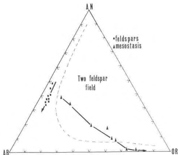
FIG. 2. Microprobe analyses of plagioclases (filled squares) and interstitial "granitic" material (filled triangles), after recalculation of the analyses into normative albite (AB), anorthite (AN), and orthoclase (OR). The limit of ternary solid solution in feldspars is taken from Carmichael (1963).
