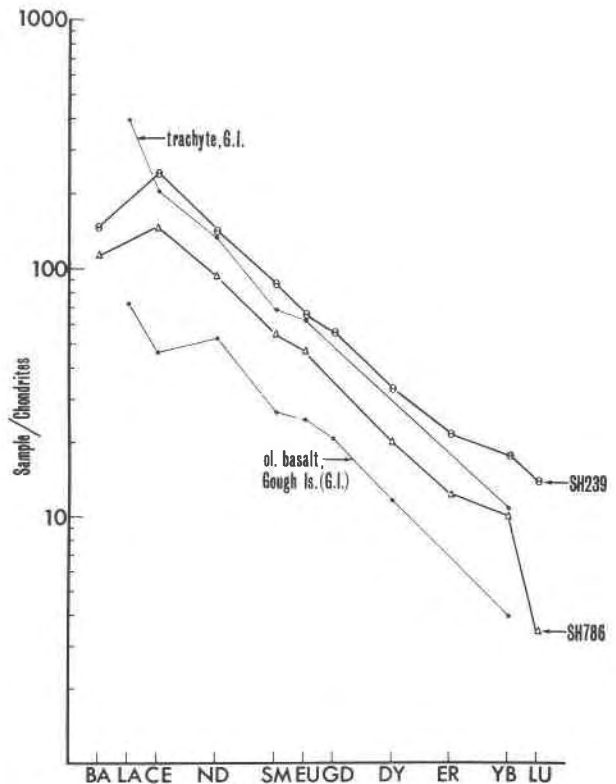
FIG. 1. Rare-earth element patterns, normalized to an average chondritic abundance, for the FHIC lava (SH239) and an alkali olivine basalt (SH786) from St. Helena. The rare earth elements were determined by isotope dilution mass spectrometry; W. I. Ridley, analyst. For comparison are plotted R.E.E. data for an olivine basalt and trachyte from Gough Island (Zielinski and Frey, 1970).
