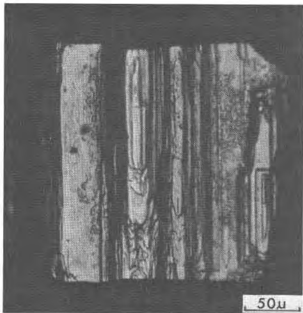
FIG. 3. Interference contrast photomicrograph of \{100\} face of a smaller crystal from the Shakanai mine, showing elongated rectangular growth layers. All photographs of crystals showing striations in this article have been reproduced in equivalent positioning, i.e. , with the vertical edges being parallel to [001] .
