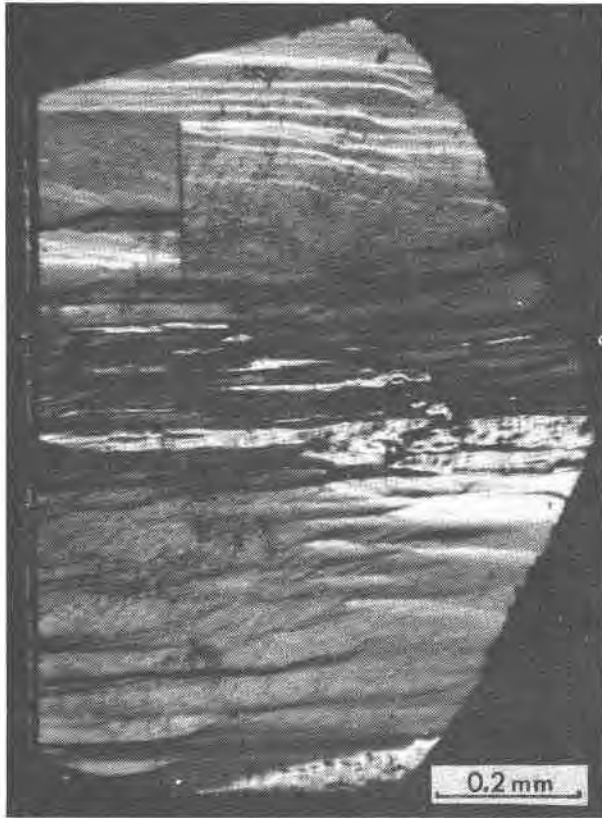
FIG. 5. Interference contrast photomicrograph of (210) face of a larger size crystal from the Shakanai mine, showing growth layers elongated parallel to the negative striations.
