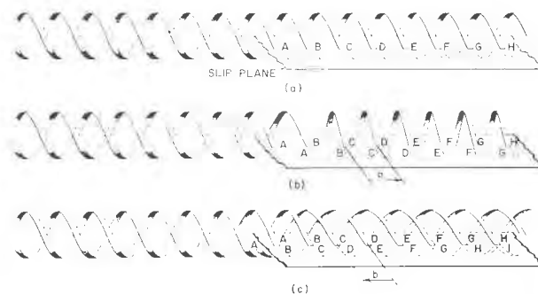
FIG. 2. (a) To introduce a screw dislocation along the axis of a high-quartz double helix, let the individual helices be scissioned at the points labelled A, B, C, etc. (b) With that part of the double helix above the slip plane held fixed in space, let the part below the slip plane be sheared to the right by a displacement equal to the Burgers vector b . (c) The dislocation introduced into (a) by a shear that is equal and opposite to that shown in (b). [Note: Some elastic relaxation from the configurations shown in (b) and (c) is expected, especially near the edge dislocations.]
