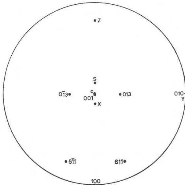
FIG. 1. The stereographic projection of the optical orientation and twinning of merwinite. Two of the twin planes, (611) and (\bar{6}\bar{1}1) , intersect at the point S , and their respective twin axes are [0\bar{1}3] and [013] . The third twin plane and cleavage on \{100\} are not shown. The angular separation between the c axis and [001] is nearly 2^\circ .
