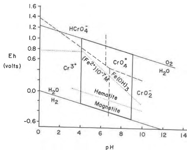
FIG. 6. Eh-pH diagram for chromium and iron species in water at 25^\circ\text{C} . Shaded dashed lines give stabilities of chromium species (Klein, 1962, diagram 23); shaded dotted lines give stabilities of some iron species (Krauskopf, 1967); heavy solid lines enclose the range of usual near-surface environments; and light solid lines delimit the stability conditions of water.
