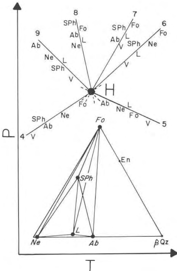
FIG. 2. Pressure-temperature projection of schematic array of univariant reactions about invariant point H. Chemo-graphic relations of invariant phases; except vapor, shown in projection from the H 2 O apex onto the NaAlSiO 4 (Ne)-Mg 2 SiO 4 (Fo)-SiO 2 (βQz) base.
