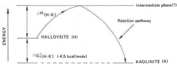
FIG. 10. Relationship between activation energy ( \Delta H_{(H-K)} ) and free energy of reaction ( \Delta G_{r(H-K)}^\circ ) for the kaolinite-halloysite system.
