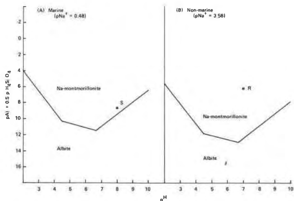
FIG. 7. Isoplethic sections of the stability diagram (Na-montmorillonite and albite) for marine (sea water) and non-marine (average river water) environments. S and R are the compositions of sea water and average river water. (A) Marine ( pNa^+ = 0.48 ); (B) Non-marine ( pNa^+ = 3.58 ).
