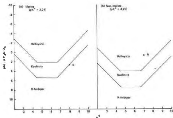
FIG. 2. Isoplethic sections of the stability diagram (K-feldspar—kaolinite and K-feldspar—halloysite) for marine (sea water) and non-marine (river water) environments. S and R are the compositions of sea water and average river water, respectively. (A) Marine ( \text{pK}^+ = 2.21 ), (B) Non-marine ( \text{pK}^+ = 4.25 ).
