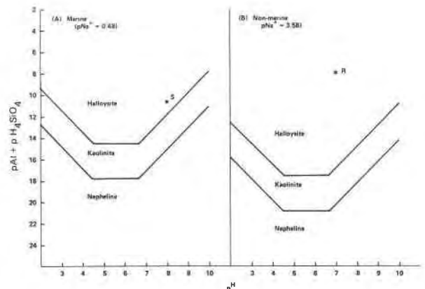
FIG. 6. Isoplethic sections of the stability diagrams nepheline-kaolinite and nepheline-halloysite for marine (sea water) and non-marine (average river water) environments. S and R are the compositions of sea water and average river water. (A) Marine ( pNa^+ = 0.48 ); (B) Non-marine ( pNa^+ = 3.58 ).
