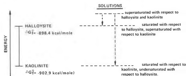
FIG. 9. Relative thermodynamic stabilities of kaolinite and halloysite.
