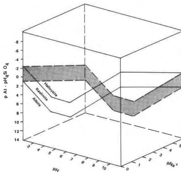
FIG. 3. Stability diagram of albite-kaolinite and albite-halloysite at 25°C and 1 atm., in which p\text{Al}-p\text{H}_4\text{SiO}_4 is plotted against pH and p\text{Na}^+ .
