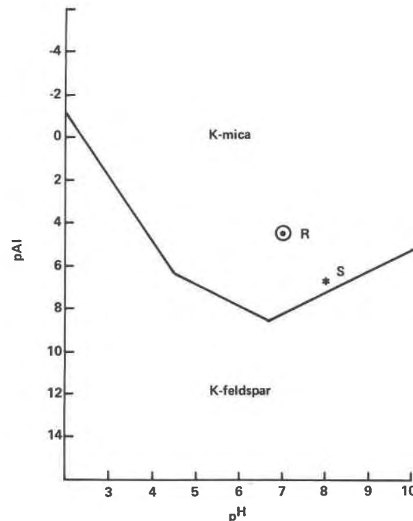
FIG. 8. Stability diagram of K-mica and K-feldspar at 25°C and 1 atm., in which pAl is plotted against pH. S and R are the composition of sea water and average river water.
