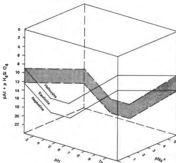
FIG. 5. Stability diagram of nepheline-kaolinite and nepheline-halloysite at 25°C and 1 atm., in which pAl + pH_4SiO_4 is plotted against pH and pNa^+ .
