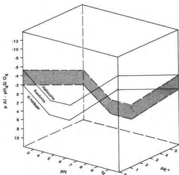
FIG. 1. Stability diagram of K-feldspar-kaolinite and K-feldspar-halloysite at 25°C and 1 atm., in which p\text{Al} - \text{pH}_4\text{SiO}_4 is plotted against \text{pH} and \text{pK}^+ .
