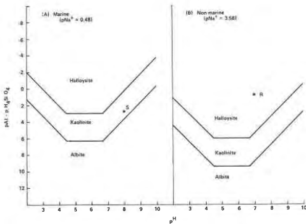
FIG. 4. Isoplethic sections of the stability diagram (albite-kaolinite and albite-halloysite) for marine (sea water) and non-marine (average river water) environments. S and R are the compositions of sea water and average river water respectively. (A) Marine ( pNa^+ = 0.48 ); (B) Non-marine ( pNa^+ = 3.58 ).
