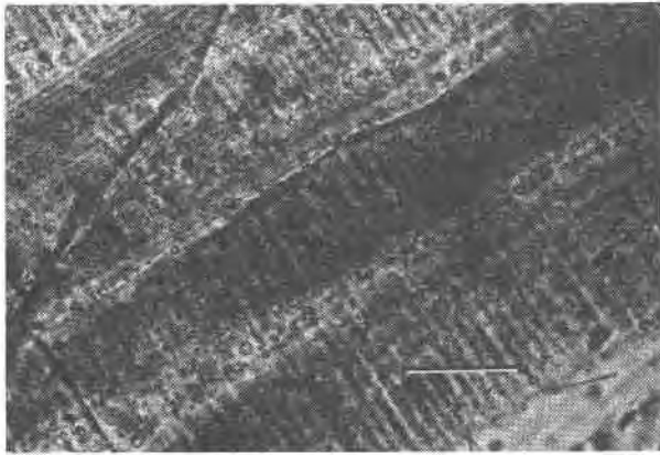
FIG. 2. Photomicrograph of iron oxide inclusions oriented parallel to twin lamellae in clouded plagioclase of metadolerite. The trace of the (010) twin plane crosses the photomicrograph from upper right to lower left. Plane polarized light. Sample A114. Bar scale measures 0.02 mm.
