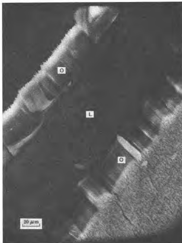
FIG. 2. Scanning electron micrograph showing fibrous layers of offretite (O) that grew normal to a single crystal of levyne (L).
