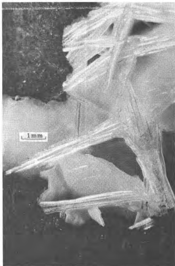
FIG. 1. Boxwork of levyne (pale gray) and offretite (white) in a large vesicle in the Picture Gorge Basalt.
