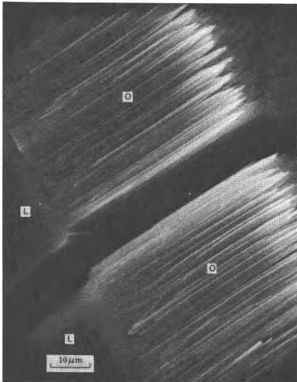
FIG. 3. Scanning electron micrograph showing the individual fibers of offretite (O) that grew normal to (0001) of levyne (L).
