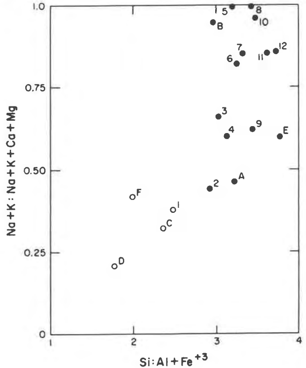
FIG. 4. Plot showing the compositional variation of erionite (black dot) and offretite (open circle). Source for the numbered analyses is Sheppard and Gude (1969). Sources for the lettered analyses are A, Batiashvili and Gvakhariya (1968); B and C, Shimazu and Mizota (1972); D, Cross and Hillebrand (1885); E, Sheppard and Gude (1973); F, this report.
