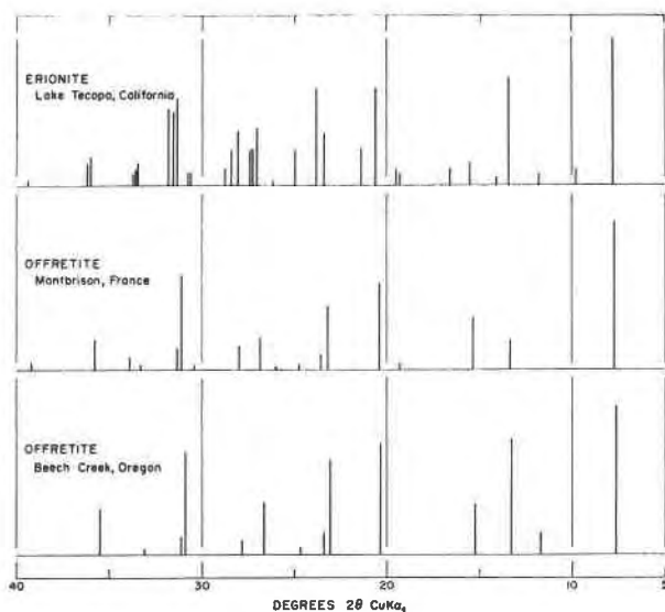
FIG. 5. Diagrammatic representation of X-ray powder diffractometer patterns for the Beech Creek offretite, the Montbrison offretite, and a typical erionite. Relative intensities are indicated by height of lines above baseline.
