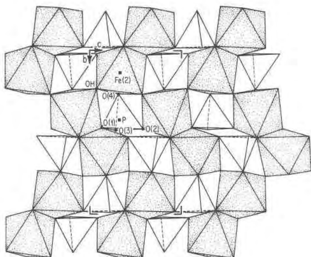
FIG. 2. Polyhedral diagram of the whitmoreite crystal structure down the z*-axis. The Fe 3+ -O octahedral sheet is stippled, and the linking [PO 4 ] tetrahedra above and below the sheet are unshaded. The Fe(1)-O octahedron between the sheets is omitted.
