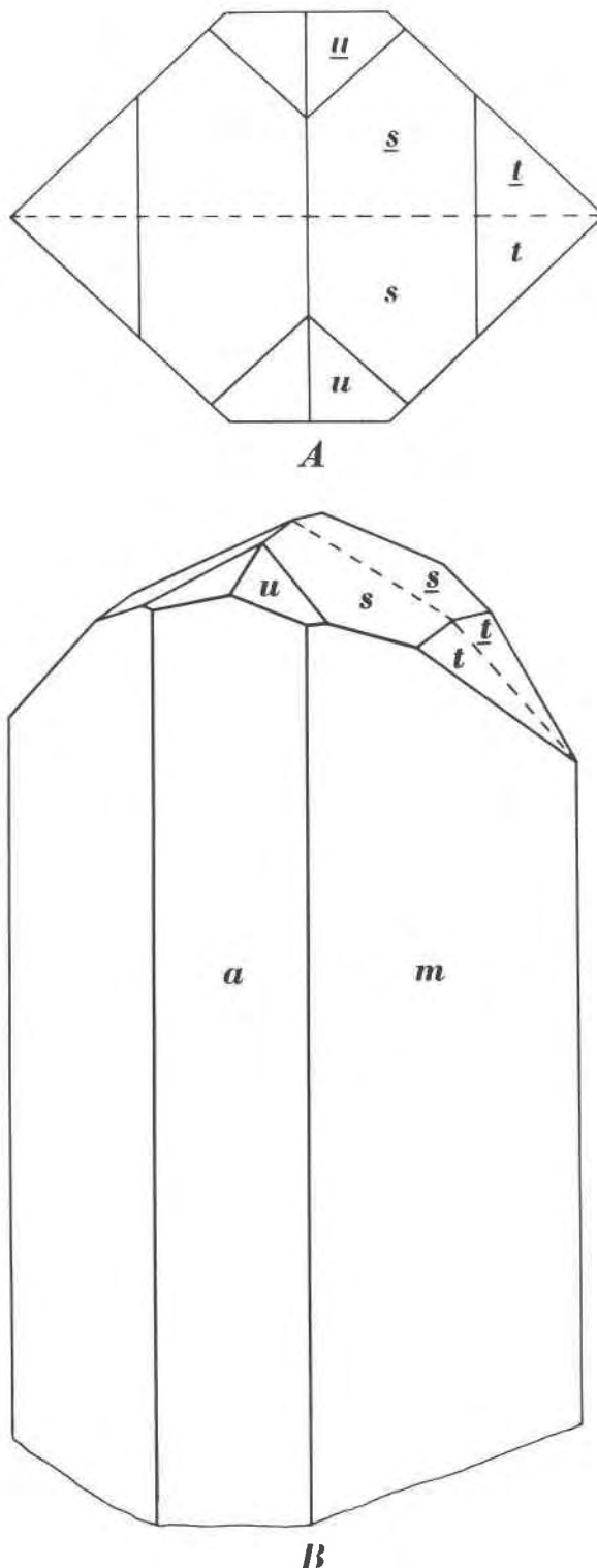
FIG. 1. Typical development of whitmoreite crystals twinned by reflection on \{100\} showing the forms a\{100\} , m\{110\} , s\{011\} , t\{021\} , and u\{112\} . A. Plan. B. Clinographic projection.
