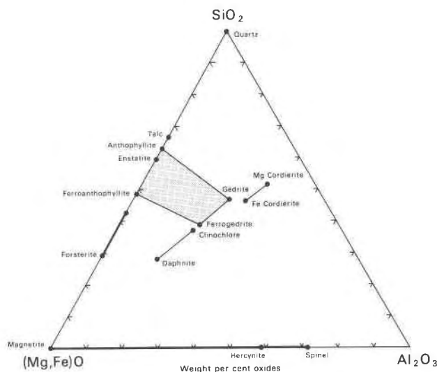
FIG. 2. Phases encountered in the experiment products.
