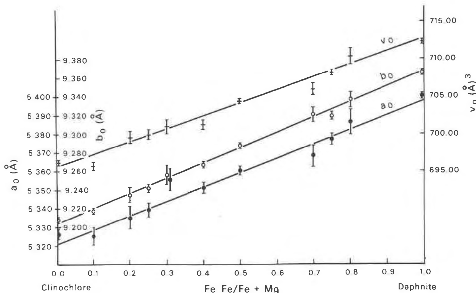
FIG. 4. Cell dimensions of synthetic chlorites on the clinochlore-daphnite join (see Table 4). Straight lines were obtained from linear regression equations—see text for correlation coefficients.
