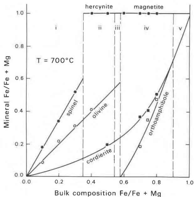
FIG. 8. Fe/Fe+Mg ratios for individual phases in the five chlorite breakdown assemblages as a function of Fe/Fe+Mg in the bulk composition. Numbers i to v are the various chlorite breakdown assemblages as in Figure 7 and all data are for experiments at 700°C and 2.07 kbar P_{H_2O} under the NNO buffer.
