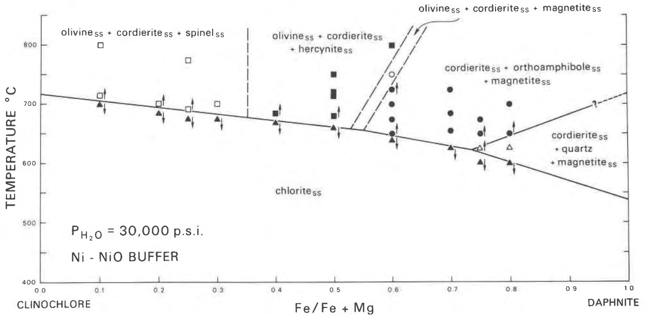
FIG. 7. T - X projection at 2.07 kbar P_{H_2O} of experimental results for the join clinocllore- Mg_5Al_2Si_3O_{10}(OH)_8 -daphnite- Fe_5Al_2Si_3O_{10}(OH)_8 under the NNO buffer. Arrows pointing to higher temperatures indicate the particular result was obtained with the lower temperature assemblage as starting material, and vice versa for arrows pointing to lower temperatures ( i.e. , indicators of reaction reversals).
