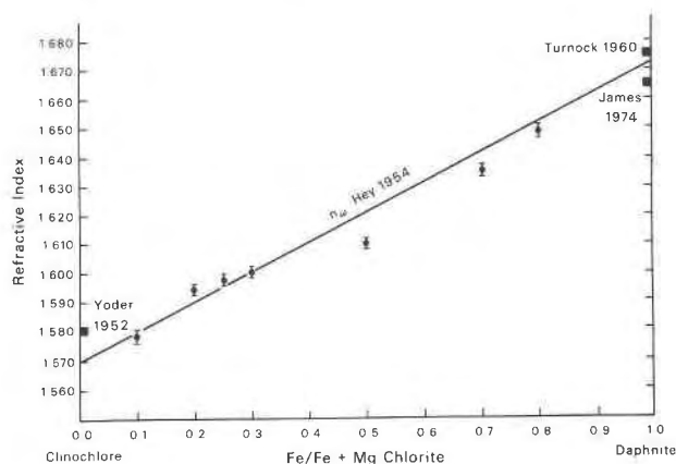
FIG. 3. Mean refractive indices of synthetic chlorites. The line derived by Hey (1954) was based on indices of natural chlorites. See Table 2.
