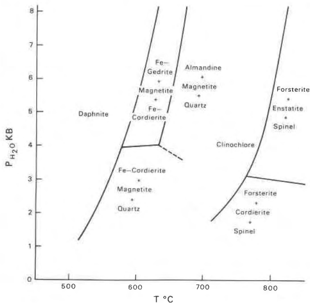
FIG. 1. Upper stability limits of clinocllore (Fawcett and Yoder, 1966) and daphnite (James et al. , 1974), the latter at the NNO buffer.
