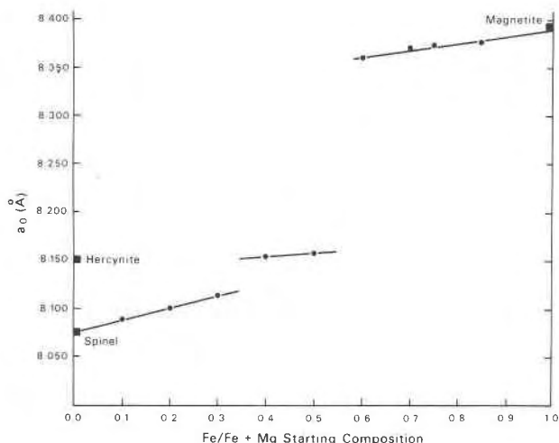
FIG. 6. Plot of estimated spinel compositions from the data of Table 12.
