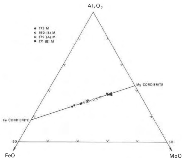
FIG. 5. Electron microprobe analyses of cordierite grains. Each point represents an average of numerous spot analyses within a single grain. Distribution of symbols indicates the compositional range of cordierites in a single experiment. (Figure in wt percent)
