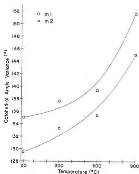
FIG. 3D. A plot of the octahedral angle variance (as defined by Robinson et al. , 1971) versus temperature for fayalite.
