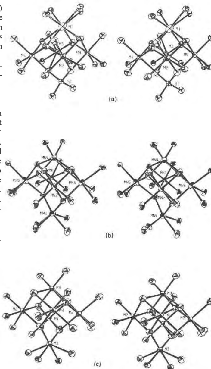
FIG. 1. Atomic arrangements around vacant sites. (a) the ( Mn^{2+}Mn_3^{3+}Si ) arrangement in braunite; (b) the ( Mn_3^{3+} ) arrangement in \alpha - Mn_2O_3 . (c) the ( Mn_3^{3+} ) arrangement in braunite.
