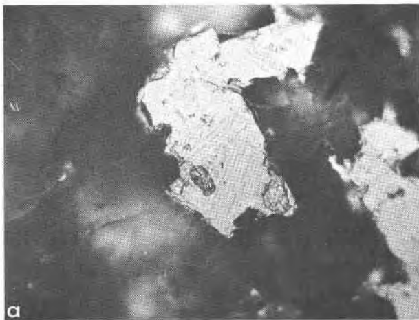
FIG. 1. Photomicrograph of highly oxidized specimen, U12-2a. (a) Deuteritic oxidation class 4 grain with small rectilinear islands of magnetite (medium gray) separated by broad off-white lamellae consisting of a fine aggregate of rutile and titanohematite. (b) Partly oxidized olivine grain containing and partly surrounded by thin (white) veins of hematite. Scale: 1\frac{1}{2} inches = 50 \mu .
