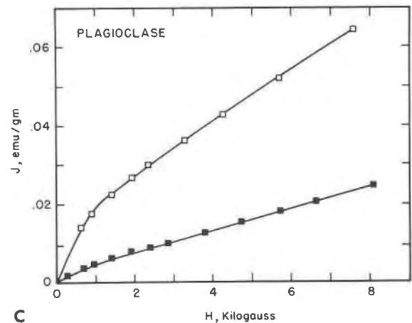
FIG. 3. Specific magnetization ( J ) vs field ( H ) curves for (a) oxide, (b) pyroxene, and (c) plagioclase concentrates from oxidized basalt (open symbols) and unoxidized basalt (closed symbols).
