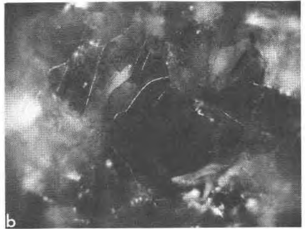
FIG. 1. Photomicrograph of highly oxidized specimen, U12-2a. (a) Deuteritic oxidation class 4 grain with small rectilinear islands of magnetite (medium gray) separated by broad off-white lamellae consisting of a fine aggregate of rutile and titanohematite. (b) Partly oxidized olivine grain containing and partly surrounded by thin (white) veins of hematite. Scale: 1\frac{1}{2} inches = 50 \mu .
