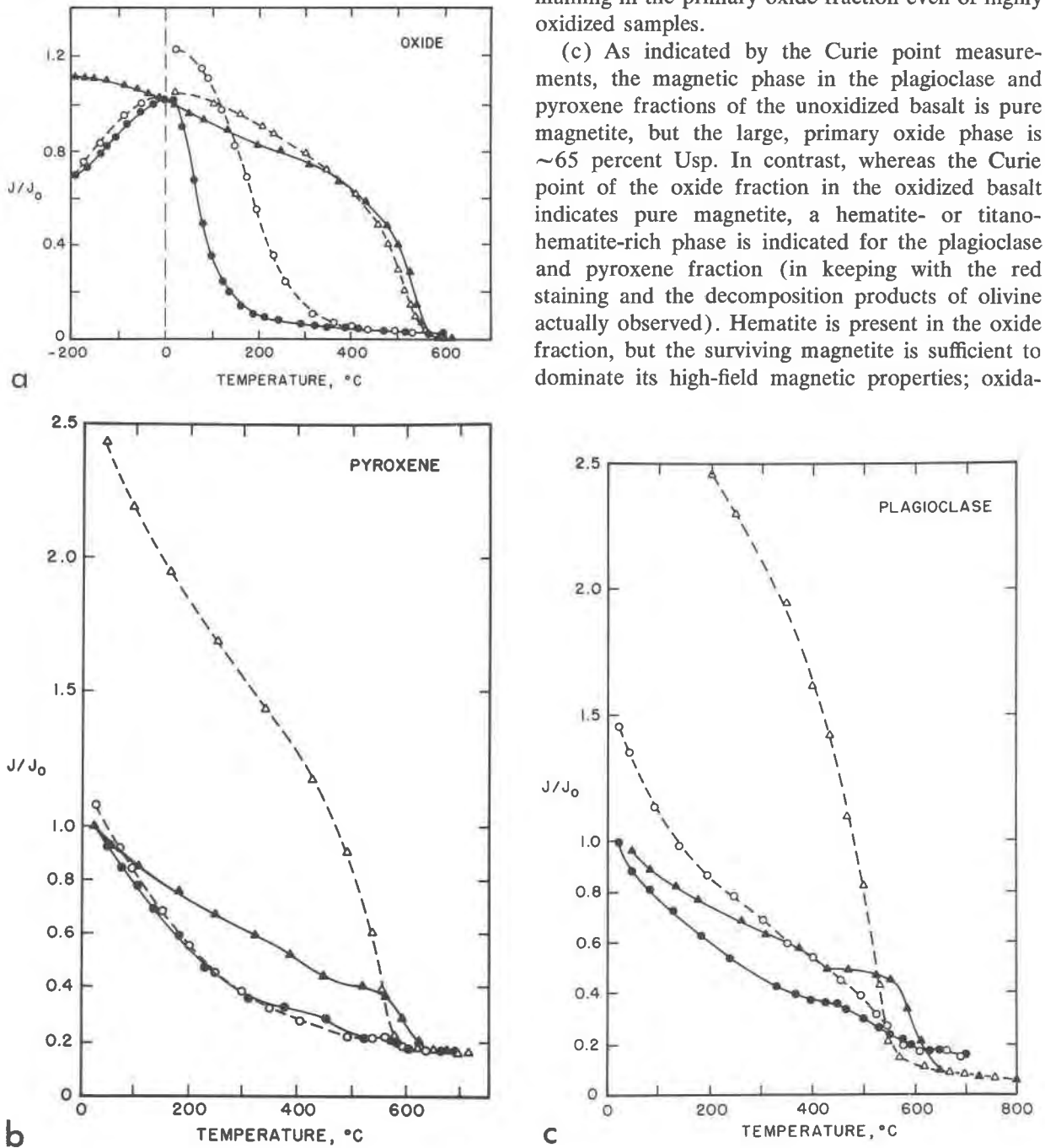
FIG. 4. Magnetization ( J ) vs temperature curves for (a) oxide, (b) pyroxene, and (c) plagioclase concentrates. Magnetizing field = 3000 gauss; initial vacuum = 2 \times 10^{-5} torr. Curves normalized to value at room temperature. Circles and triangles pertain to unoxidized and oxidized samples, respectively; solid symbols for heating and open symbols for cooling cycles.
