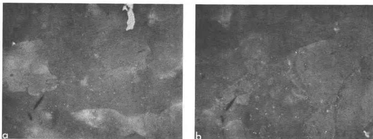
FIG. 2. Photomicrograph of unoxidized specimen, U16-1a. (a) Large primary ulvöspinel-rich titanomagnetite (light grain in upper right) and many examples of the small-sized form of magnetite (light specks). Note the strong partitioning of the small-sized magnetite into the darkest silicate phase, which is plagioclase feldspar. (b) The small-sized magnetite (white specks) is again largely restricted to the plagioclase (dark gray), but also occurs as inclusions within and along the boundaries between the pyroxene grains (medium gray). Scale same as Figure 1.
