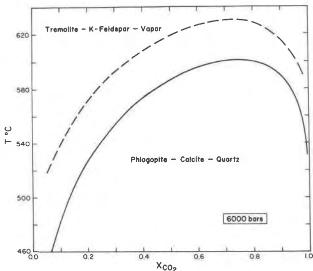
FIG. 3. T - X curve at 6 kbar calculated from the \log f_{\text{CO}_2} f_{\text{H}_2\text{O}}^2 - 1/T plot in Figure 2. Ideal mixing has been assumed for the fluid. The dashed curve represents the data of Hoschek (1973).
