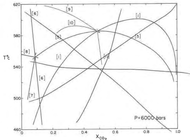
FIG. 4. Phase relations at 6 kbar involved at the intersection of the following equilibria for which some experimental data are available:
