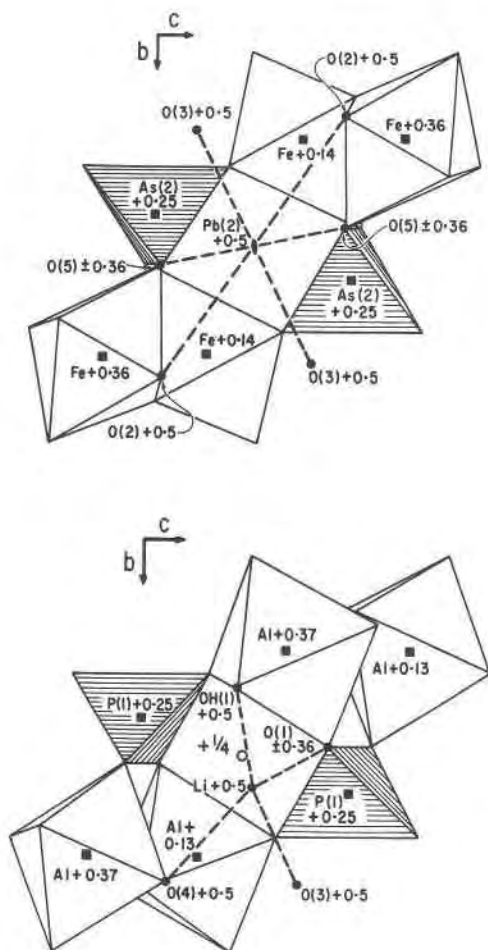
FIG. 3. The polyhedral environments of Pb(2) in carminite (top) and Li in palermoite (bottom) down the a axis. The Pb(2) atom resides at (1/2 \ 1/4 \ 1/4) . In palermoite, the locus at (1/4 \ 1/4 \ 1/4) is drawn as a circle.
