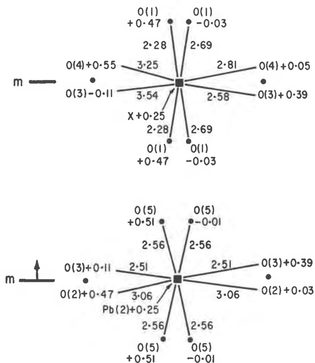
FIG. 4. The "X"-O bonds and Pb(2)-O bonds in palermoite (top) and carminite (bottom). The symmetry elements ( m and 2/m respectively) are shown on the left and apply to the loci of "X" and Pb(2). Bond distances are specified.
