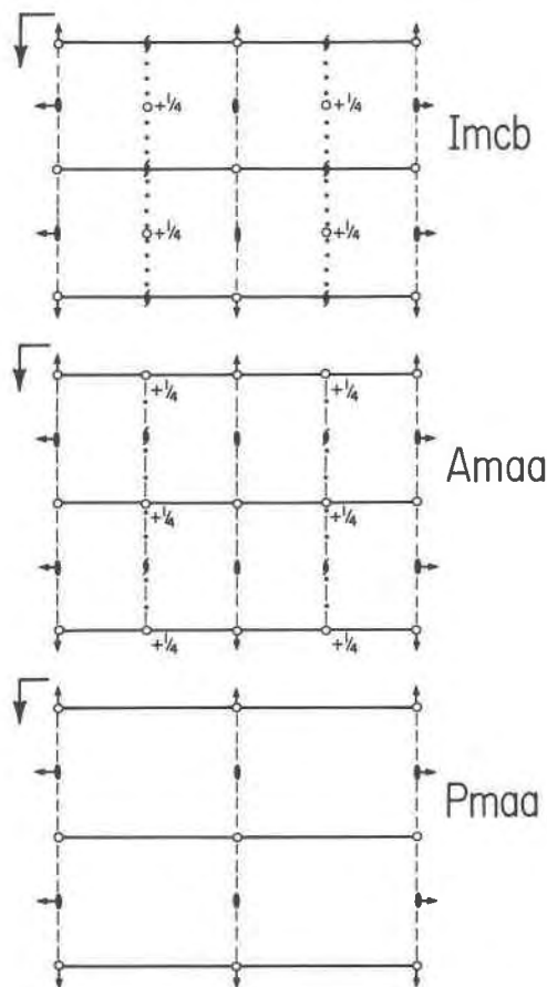
FIG. 1. Symmetry diagrams of the space groups Imcb , Amaa , and Pmaa in standard cell orientation (down the c axis). The first two groups apply to palermoite and carminite respectively. The third group is the subgroup common to the first two.
