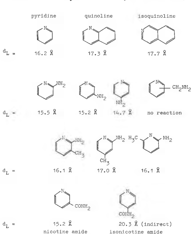
FIG. 5. Basal spacings d_L of H-magadiite intercalation compounds with pyridine derivatives.
