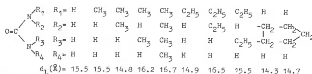
FIG. 9. Basal spacings of H-magadiite-urea intercalation compounds.
