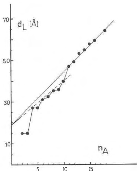
FIG. 10. Basal spacings d_L of the n -alkylamine-DMSO intercalation complexes of H-magadiite. ( n_A is the number of carbon atoms in the alkyl chain).
