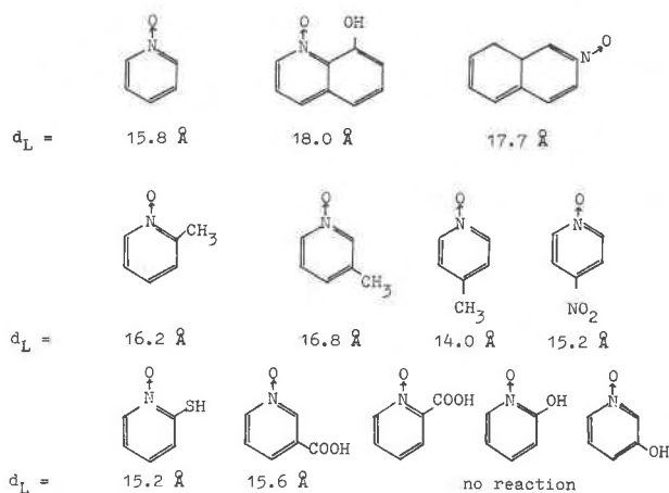
FIG. 3. Basal spacings d L of H-magadiite intercalation compounds with pyridine-N-oxides.
