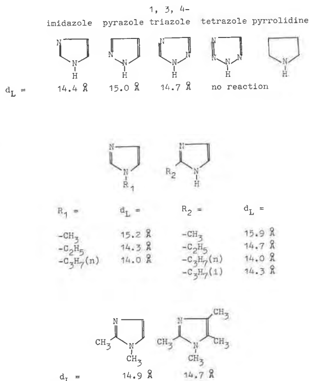
FIG. 6. Basal spacings d_L of H-magadiite intercalation compounds with 5-ring heterocycles.
