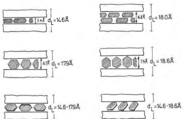
FIG. 4. Arrangements of aromatic rings between the layers of H-magadiite and resulting maximal basal spacings d_L .
