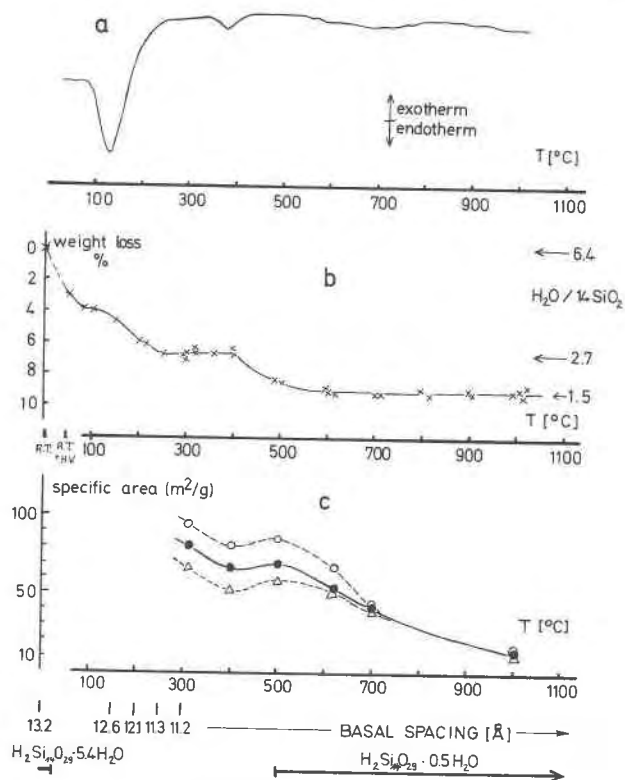
FIG. 1. Thermal behavior of H-magadiite. (a) DTA-curve; (b) weight loss curve; (c) variation of specific area with preheating temperature measured with oxygen (○), nitrogen (●) and argon (Δ) by gas adsorption at -196°C.
