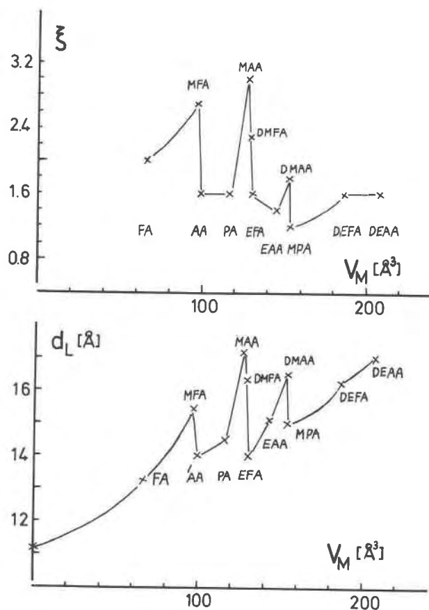
FIG. 8. Basal spacings d_L and limiting composition \xi (moles/14 \text{SiO}_2 ) of acid amide intercalation complexes as function of molecular volume V_M of acid amides. (FA = formamide, AA = acetamide, PA = propionamide, MFA = methylformamide, DEAA = diethylacetamide, etc).
