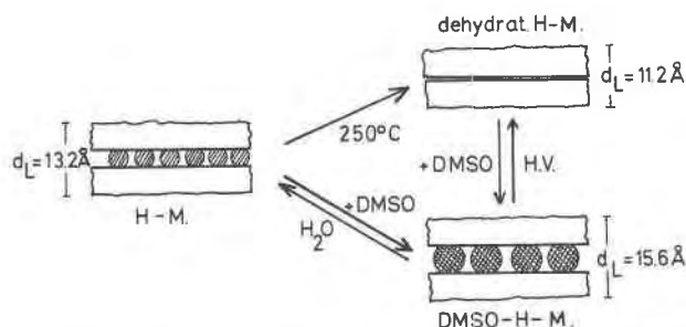
FIG. 2. Schematic representation of intercalation reactions of H-magadiite (H-M) with dimethylsulfoxide (DMSO).
