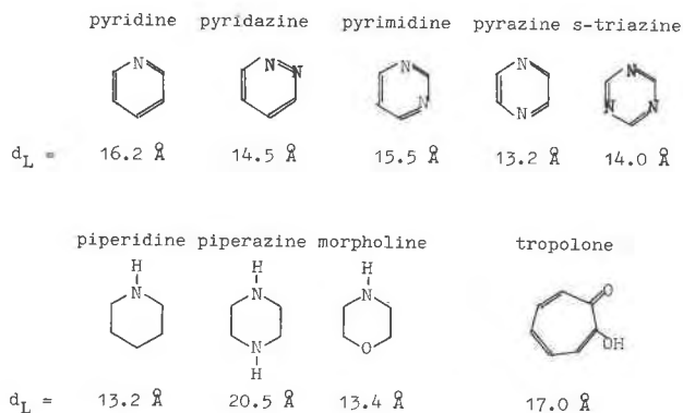
FIG. 7. Basal spacings d_L of H-magadiite intercalation compounds with 6-ring and 7-ring heterocycles.
