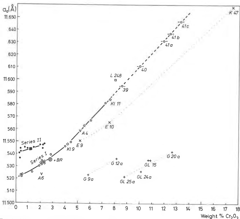
FIG. 3. Cell edges of the Stockdale garnet fractions (series I and II) plotted against chromium content. For comparison, plots of other pyrope garnets are added. (1) chromium-rich garnets from garnet peridotites: K19 and K11 (Kleinpöchlarn, Austria); L248 (Drilling T7, Linhorka, Bohemia) (Rost and Grigel, 1969). (2) Kimberlite garnets: (a) BR ("red garnet", Brookins et al. , 1966, 1967; from Stockdale); (b) A6 and A4 (O'Hara and Mercy, 1963); (c) E9, E10, and K47 (Nixon et al. , 1963, 1968); (d) G9a, G12a, GL15e+h, G20a, GL24a, and GL25a (Meyer and Boyd, 1972).
