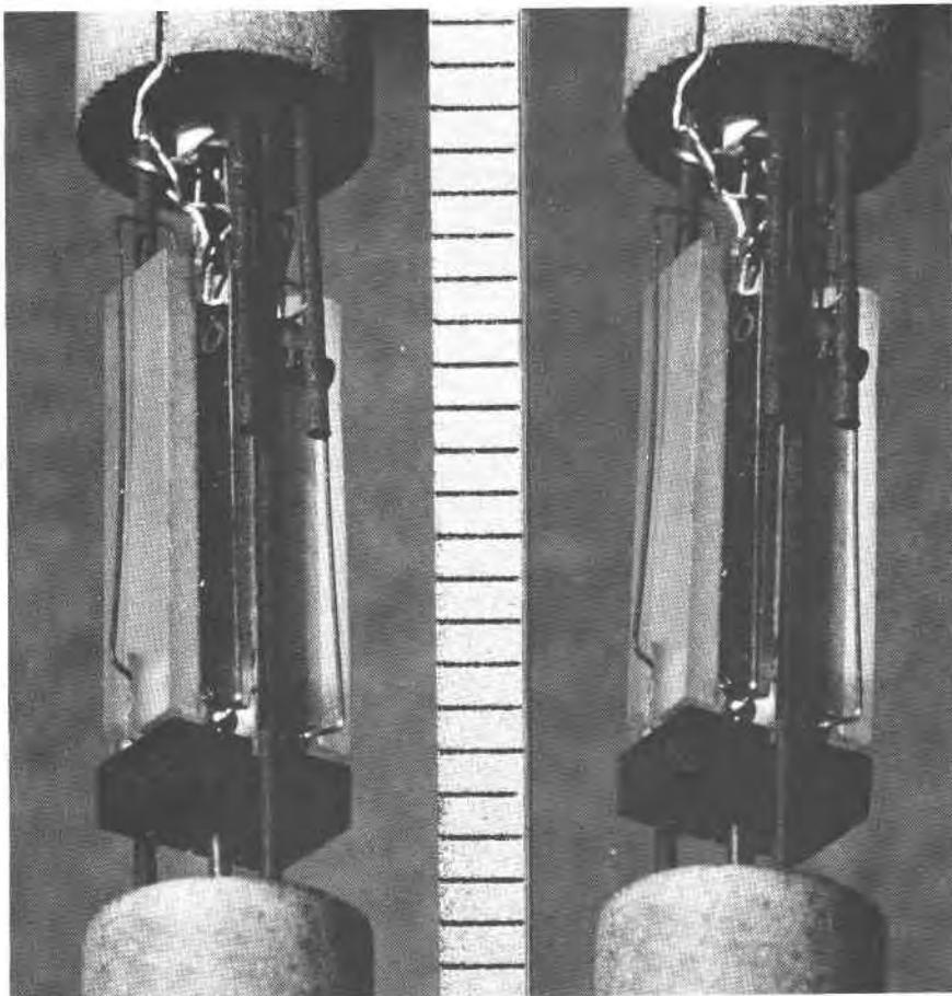
FIG. 5. Stereoscopic photograph of "gate"-type comparison dilatometer. Units on scale are millimeters. See Figure 6 for identification of parts.
