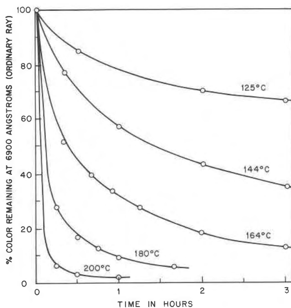
FIG. 6. Loss of Maxixe-type blue color in beryl #446 on heating at different temperatures; percent color = 100 \alpha/\alpha_0 .
