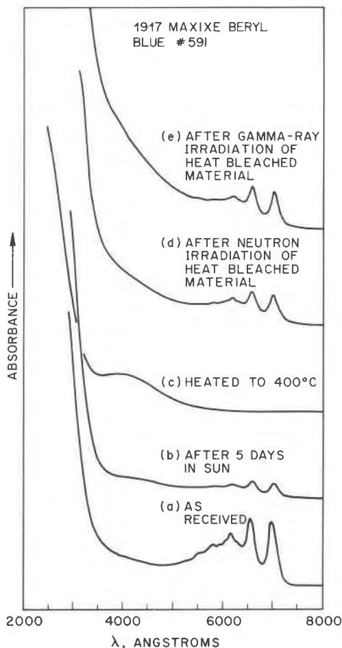
Fig. 8. Spectra of 1917 Maxixe beryl, showing the effect of light, heat, and irradiation; ordinary ray.
