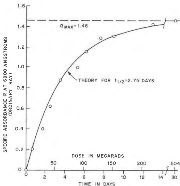
FIG. 5. Development of Maxixe-type blue color in beryl #446 during gamma-ray irradiation; points experimental, line theory.
