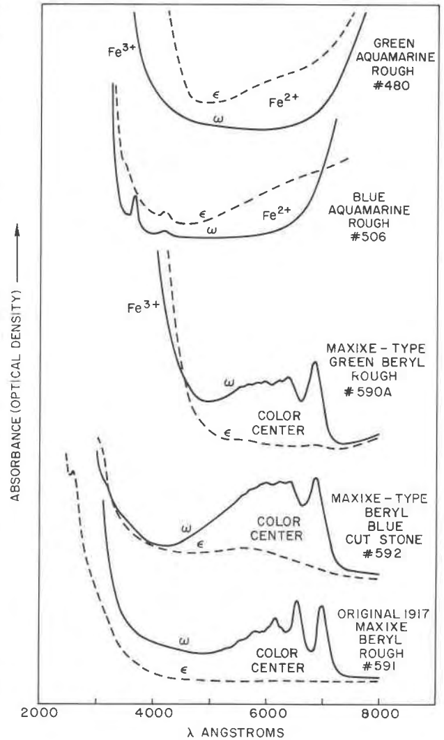
FIG. 1. Spectra of Maxixe-type beryls and aquamarines; \omega is the ordinary ray spectrum, \epsilon the extraordinary ray spectrum. Absorbance = \log_{10}(I_0/I) .
