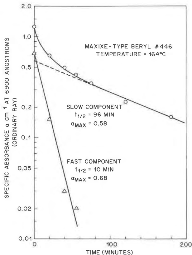
Fig. 7. Decomposition of the 164°C heat-bleaching curve of Figure 6 into two exponential components; points experimental, lines theory.
