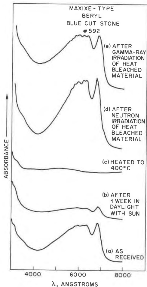
FIG. 4. Spectra of blue Maxixe-type beryl (cut stone immersed in carbon tetrachloride in quartz cell) showing the effect of light, heat, and irradiation; ordinary ray.
