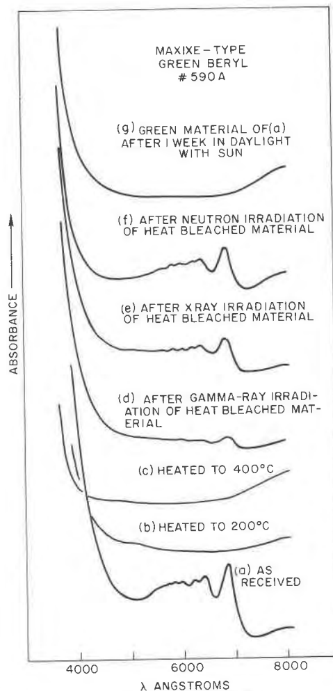
FIG. 3. Spectra of green Maxixe-type beryl showing the effect of light, heat, and irradiation; ordinary ray.
