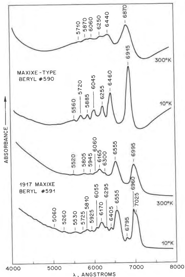
FIG. 2. Spectra of Maxixe and Maxixe-type beryl, ordinary ray, at 300 K and 10 K.
