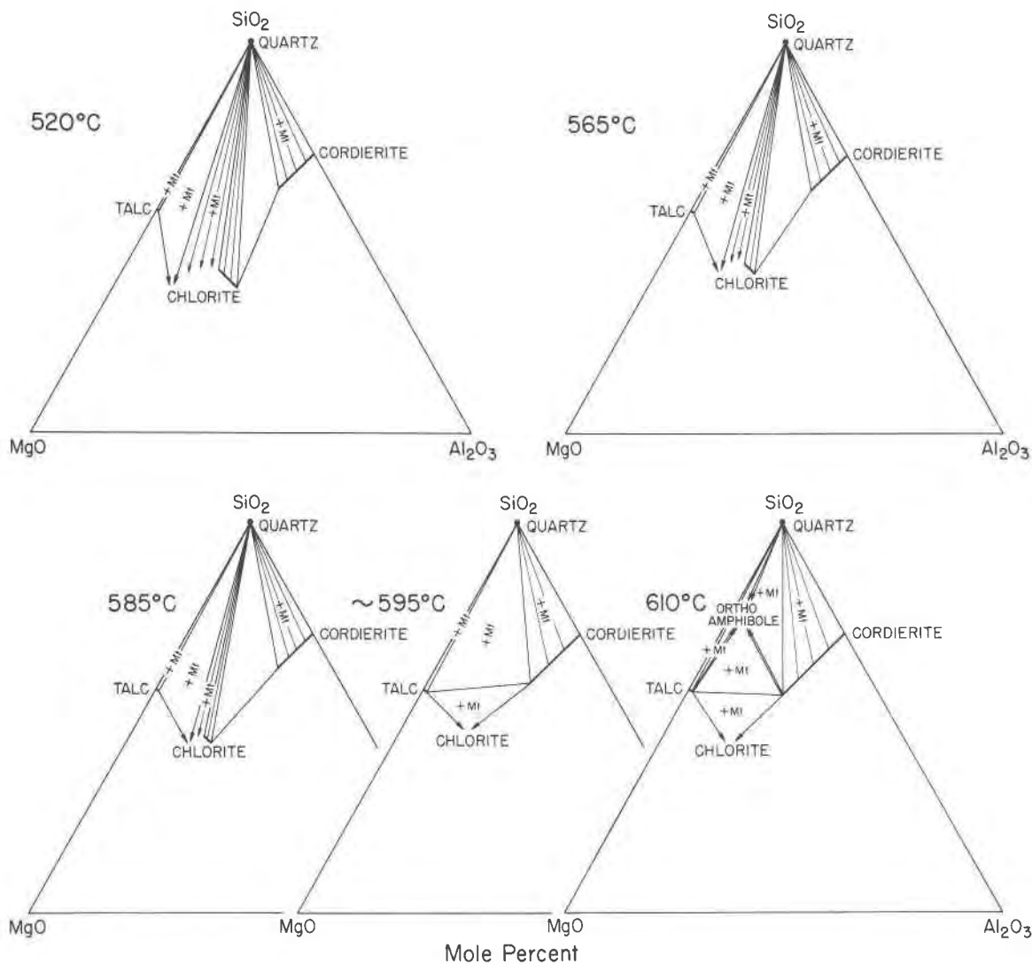
FIG. 8. Isothermal projections from FeO-H 2 O in the Ni/NiO-buffered system MgO-FeO-Al 2 O 3 -SiO 2 -H 2 O at P H 2 O = 2 kbar, for bulk compositions with Fe/(Fe + Mg) = 0.5. With the exception that some data of McOnie et al. (1975) have been incorporated on the low MgO side of the diagrams, the projections illustrate only the phase relations interpreted from Figs. 5 and 7, and are therefore grossly incomplete. Chlorites in equilibrium only with quartz (heavy line) have Fe/(Fe + Mg) = 0.5. The assemblages near the left and right sides of the diagrams also contain magnetite as indicated.
