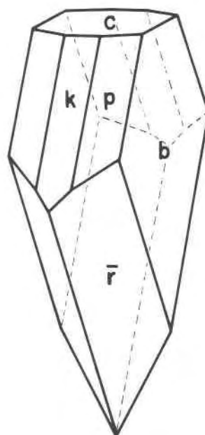
FIG. 1. Typical junitoite crystal.
