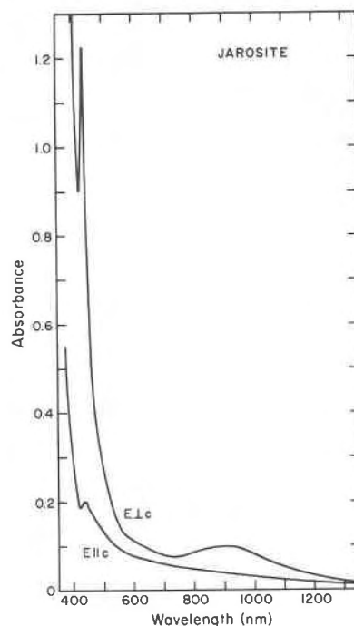
FIG. 6. Optical absorption spectrum of a jarosite crystal 22 \mu\text{m} thick from Pershing County, Nevada.
