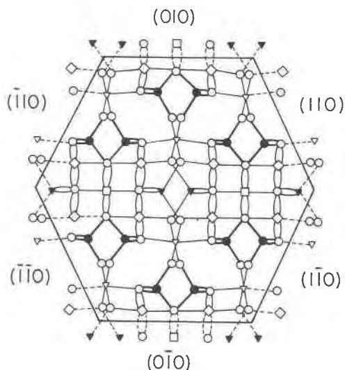
FIG. 4. Projection of the staurolite structure down [001] . Note added in proof. A more plausible surface of least bonding for \{010\} would curve around the \text{SiO}_4 groups, intersecting only Al(1)-O bonds. This change would not affect the morphology predicted in Part I, or the analysis in this paper, except that Al(1) rather than Al(2) sites would be exposed.
