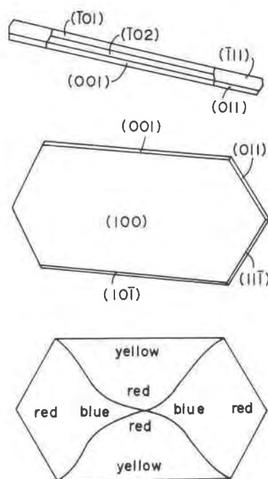
FIG. 9. Sector zoning in epidote, after Shannon (1924). The lower figure shows the birefringence observed on the flat-lying plate.
