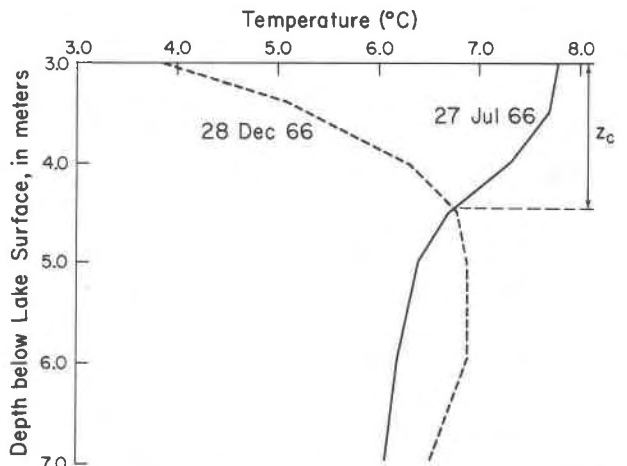
FIG. 3. Temperature profile of two thermal-probe measurements made in the sediments of Lake Waiau.
