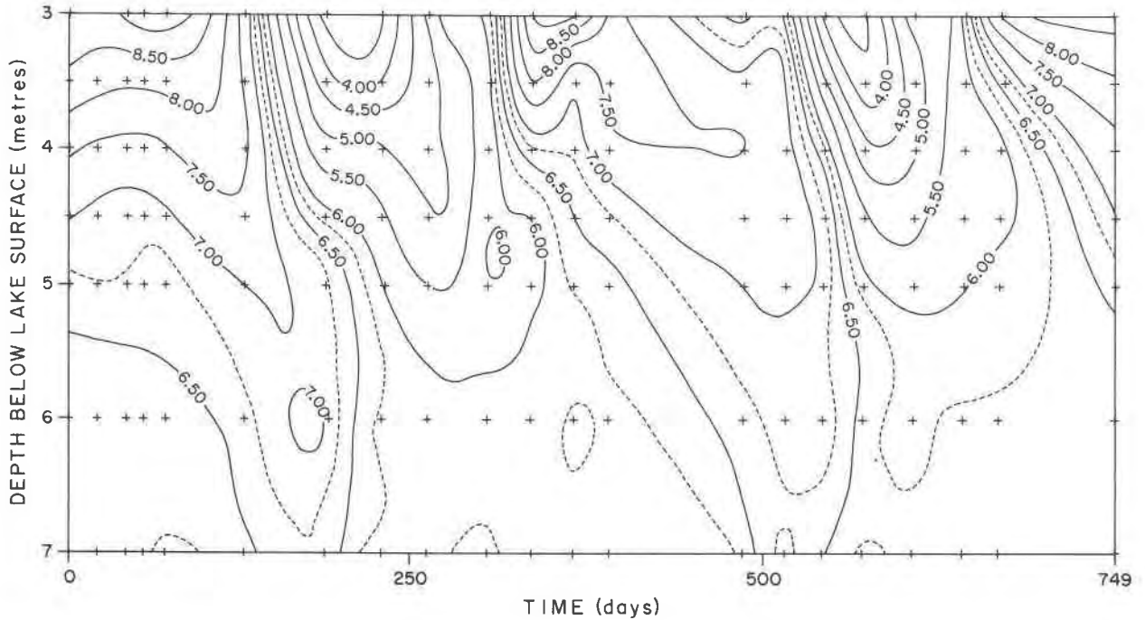
FIG. 4. Map of the temperature-probe measurements on the time-depth plane. Isothermal contours are shown.
