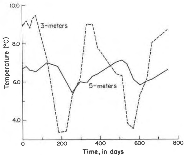
FIG. 2. Temperature, from thermal probes in Lake Waiau sediment, plotted against time for measurements taken at three and five meters below the water surface.
