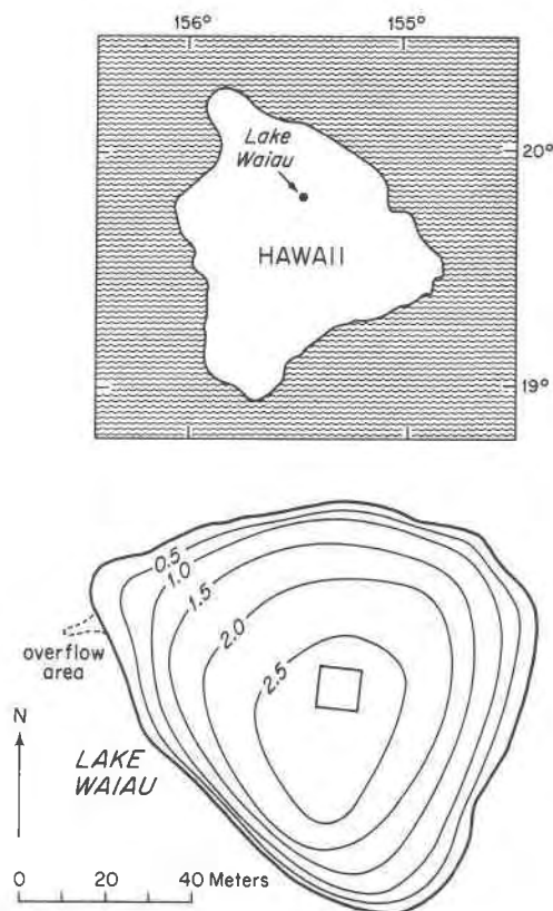
FIG. 1. Map of Lake Waiau showing estimated depth contours in meters. The inner square marks the limits of the area in which the temperature measurements were made, after Woodcock and Groves (1969).
