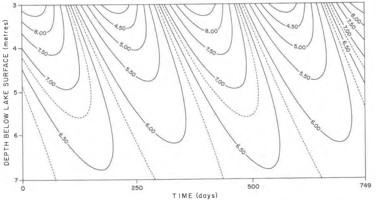
FIG. 5. Idealized map on the time-depth plane, using the values of parameters that best-fit the data in Fig. 4.
