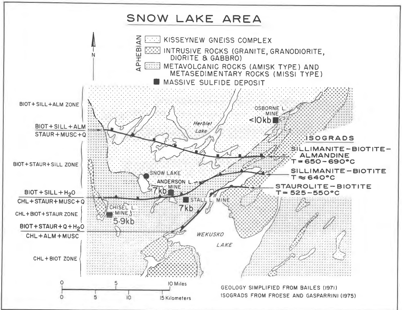
FIG. 7. Metamorphic geology of the Snow Lake area, Manitoba. Isograds mapped by Froese and Gasparrini (1975) are superimposed on a simplified version of Bailes' (1971) geological map. Isograd temperatures are estimated from Bird and Fawcett (1973), Winkler (1974) and Holdaway (1971). Pressures for four massive sulfide ore deposits are from Table 1.
