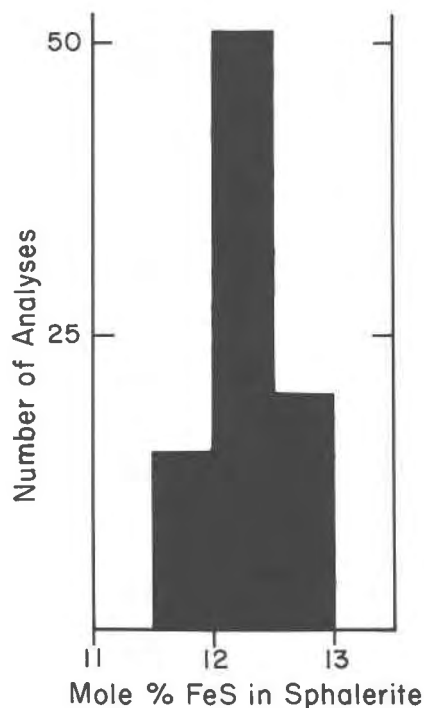
FIG. 2. Histogram of analyses of sphalerite buffered by pyrite + pyrrhotite (+ chalcopyrite) from the Geco massive sulfide orebody, Manitouwadge, Ontario. The 86 analyses from 18 polished sections give a mean of 12.19 mole percent FeS and a sample standard deviation of 0.49 mole percent FeS.
