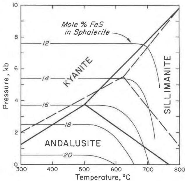
FIG. 6. P - T projection of sphalerite isopleths from FIG. 1 superimposed on the Al_2SiO_5 diagrams of Holdaway (1971, solid lines) and Richardson et al. (1969, dashed lines).
