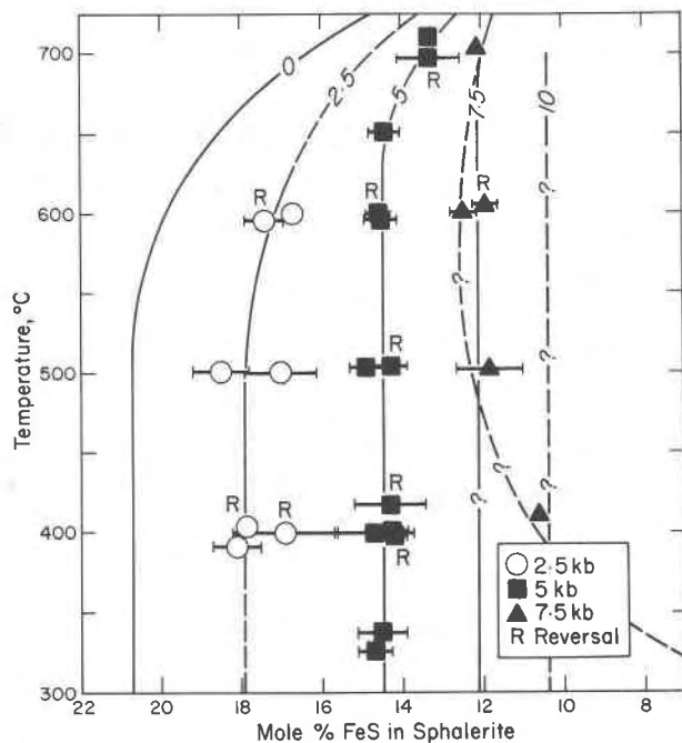
FIG. 1. T - X projection onto the FeS-Zns join of sphalerite + pyrite + hexagonal pyrrhotite isobars (in kbar), modified from Scott (1973). The vertical 7.5 kbar isobar is preferred (see text). Sphalerite + pyrrhotite and sphalerite + pyrite coexist to the left and right, respectively, of each isobar.
