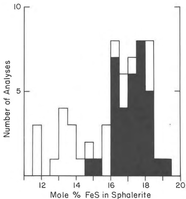
FIG. 3. Histogram of sphalerite analyses from two assemblages, Anvil mine, Yukon. Filled boxes represent 34 analyses for sphalerite coexisting with pyrite + pyrrhotite giving a mean of 17.3 mole percent FeS and sample standard deviation of 1.0 mole percent FeS. Empty boxes represent 23 analyses for sphalerite coexisting with pyrite only giving a mean of 14.9 mole percent FeS and sample standard deviation of 2.1 mole percent FeS. Data are from Campbell and Ethier (1974).
