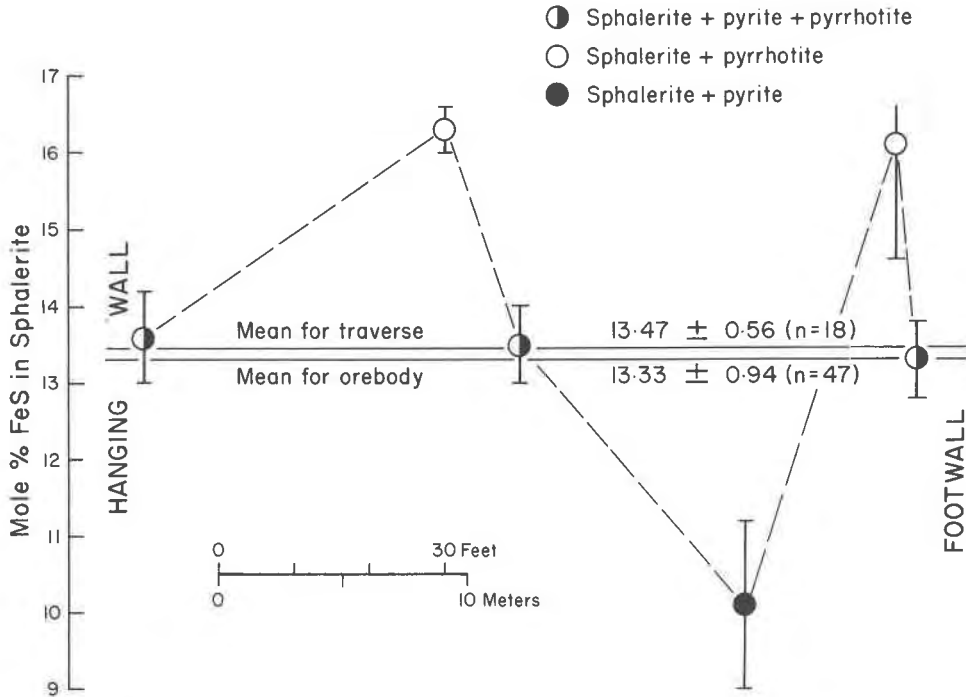
FIG. 5. Sphalerite analyses from three assemblages in a traverse through massive sulfide ore of the Fox Lake mine, northern Manitoba. Data are from this study. Vertical bars represent one standard deviation in mole percent FeS of 2 to 10 analyses at each sampling point. Means for the traverse and the orebody as a whole refer to mole percent FeS in sphalerite buffered by pyrite + pyrrhotite and exclude the other two assemblages. For both means, the standard deviation refers to a population of n analyses.
