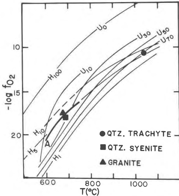
FIG. 2. F_{O_2} - T diagram for the iron-titanium oxides. Calibration curves represent the hematite content of ilmenite solid solutions and the ulvöspinel content of magnetite solid solutions as given by Buddington and Lindsley. Filled symbols represent the compositions of coexisting phases from the various lithologies. Curve A is the f_{O_2} - T conditions for the Albany quartz syenite and Conway granite samples as defined by the assemblage olivine-quartz-magnetite.
