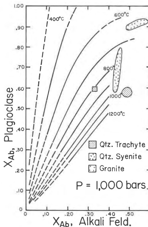
FIG. 3. Albite distribution between coexisting feldspars. Temperature calibration curves from Stormer (1975). Feldspar compositions determined as described in the text.
