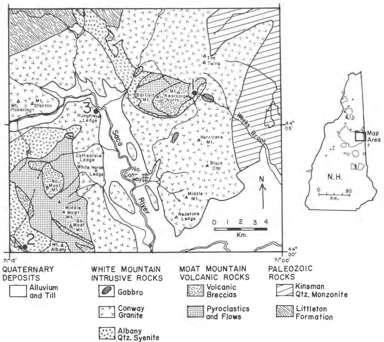
FIG. 1. Bedrock geology of a portion of the North Conway quadrangle, New Hampshire. Geology after Billings (1928). Sample locations: 1 Quartz trachyte flow, member of the Moat Mountain volcanics; 2. Albany quartz syenite; 3. Hornblende and fayalite-bearing member of the Conway granite.
