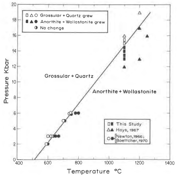
FIG. 3. Pressure-temperature diagram comparing the results obtained in this study for Gr + Qz = An_{100} + Wo with results of Newton (1966), Hays (1967), and Boettcher (1970).
