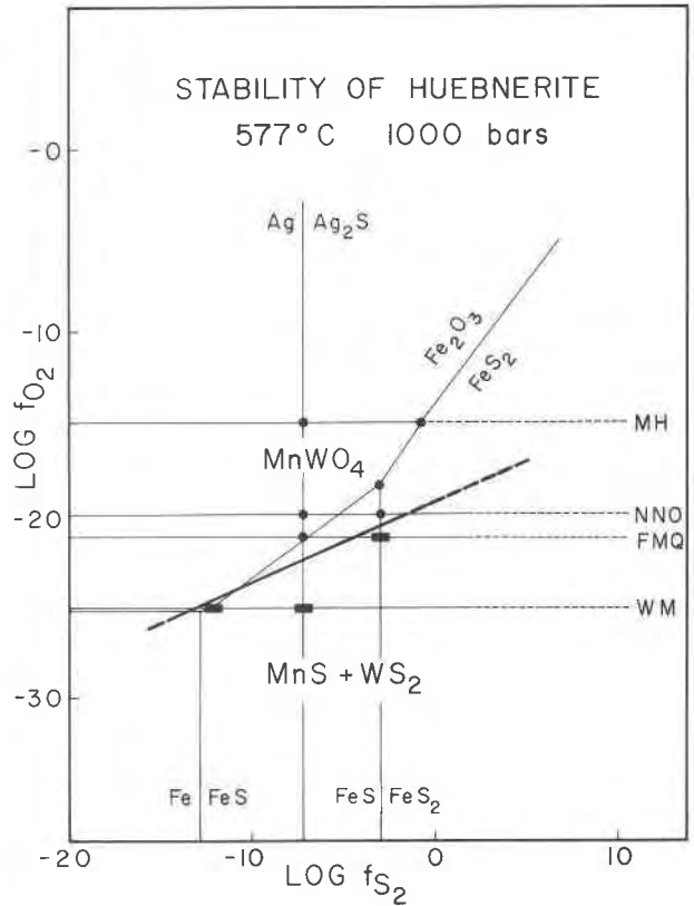
FIG. 8. The stability of huebnerite as a function of f_{O_2} and f_{S_2} at T = 577^\circ C and P_f = 1000 bars.
