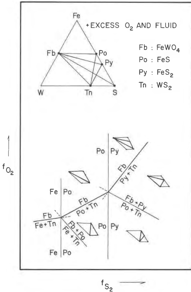
FIG. 7. The f_{O_2} - f_{S_2} relations of the phases in the system Fe-W-O-S.
