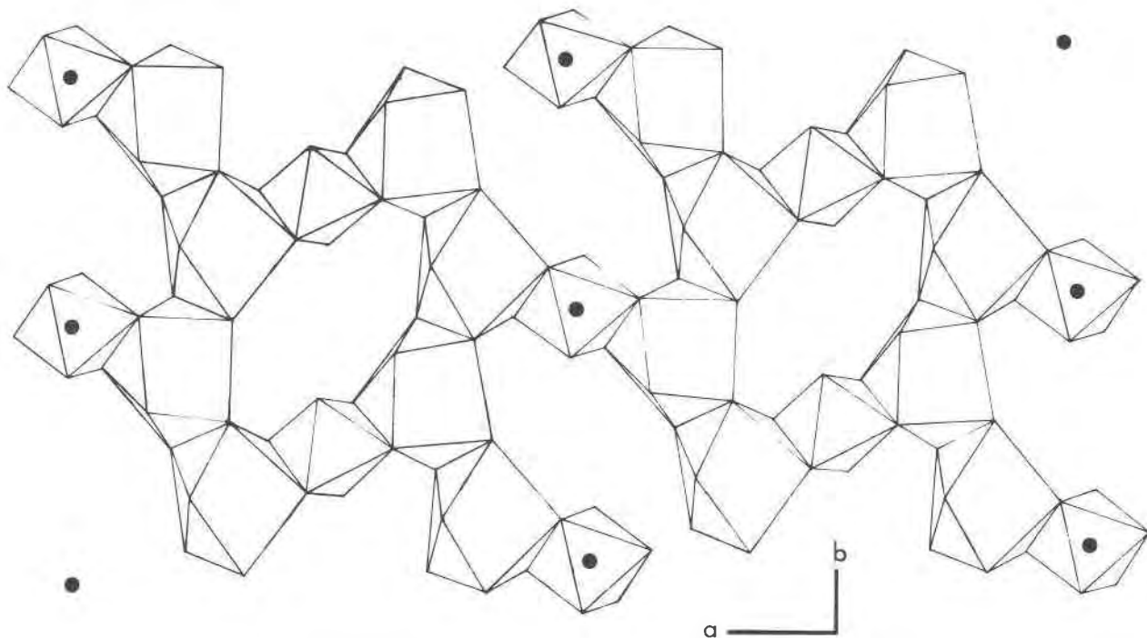
FIG. 4. The polyhedral Ca-Sn sheet in eakerite. Spots indicate Sn at unit cell corners.
