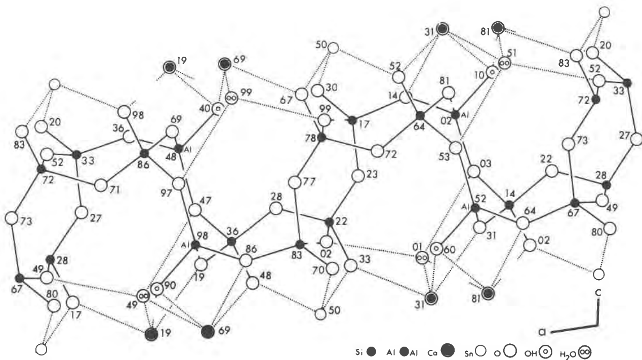
FIG. 2. The structure of eakerite, viewed down b . Numbers give the atomic coordinates, in percent, along b . Bonds within the tetrahedral network are indicated by solid lines; other bonds, including hydrogen bonds, by dotted lines. Hydrogen bonds to hydroxyl are not included because of drafting difficulties. Broken lines indicate bonds between atoms in adjacent unit cells.
