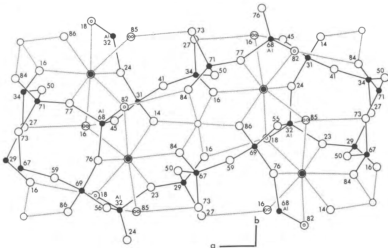
FIG. 3. The structure of eakerite, viewed down c . Numbers give atomic coordinates, in percent, along c . Bonds within the tetrahedral network are indicated by solid lines; other bonds, including hydrogen bonds, by dotted lines.
