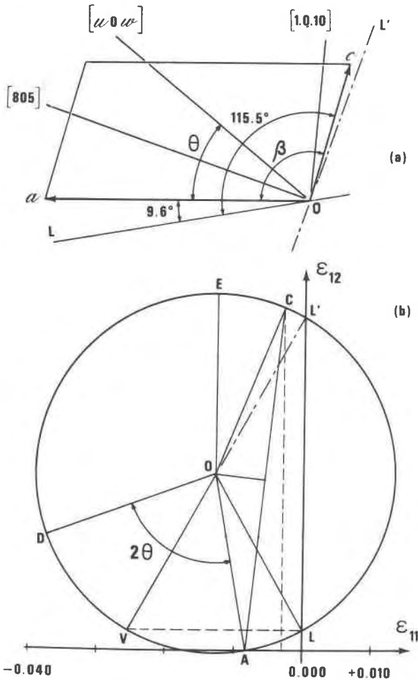
Fig. 1. (a) a c plane of clinopyroxene unit-cell. Parameters are those of an augite crystal described by Jaffe and Jaffe (1973) and cited by Robinson et al. (1971, Table 3, example 4 and Table 5). (b) Mohr circle (MC) for the lattice strain between the augite host and the pigeonite lamellae. Construction is explained in Appendix A. Points on the MC correspond to lattice directions in the crystal: A and C correspond to [100] and [001] respectively; E corresponds approximately to [1.0.10] , which is thus the lattice direction that undergoes the largest angular deviation between the two lattices; [805] (V on the MC) on the contrary has the same direction in the two lattices.
