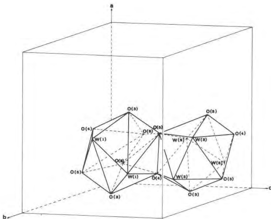
FIG. 3. The coordination polyhedra of RE(1) and RE(2) atoms.
