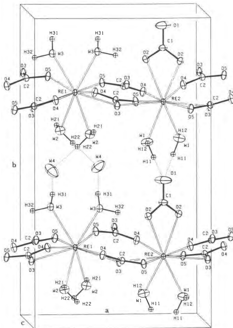
FIG. 2. ORTEP plot of the crystal structure of lanthanite showing the connection among adjacent layers of RE-O polyhedra.
