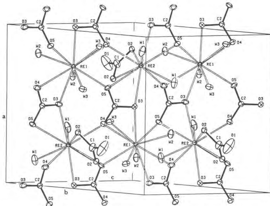
FIG. 1. ORTEP (Johnson 1965) plot of the crystal structure of lanthanite.
