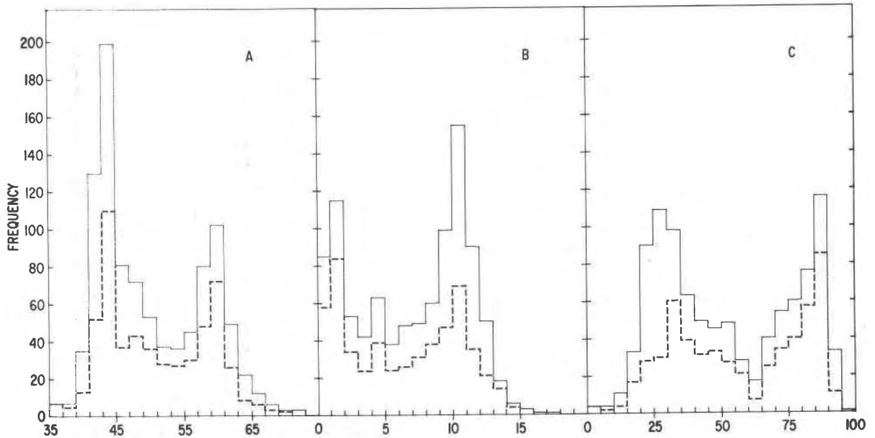
Fig. 2. Distribution of \text{SiO}_2 (A), CaO (B), and Thornton-Tuttle index (C) in analyses of volcanic rocks of the Canary Islands. Solid line—979 specimens from all islands; broken line—556 specimens from Gran Canaria, Tenerife, and La Palma only.
