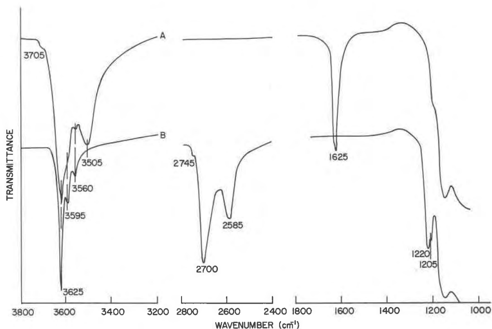
Fig. 2. Spectra of palygorskite under vacuum with structural hydroxyls as OH and coordinated water as (A) H 2 O and (B) D 2 O.
