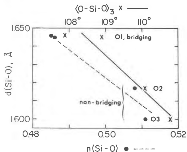
Fig. 3. Plots of the observed Si-O bond lengths, d(\text{Si-O}) , in diopside versus n(\text{Si-O}) (solid dots, dashed line) and the mean of the three O-Si-O angles, \langle O-Si-O \rangle_3 , common to the bond (X's, solid line).
