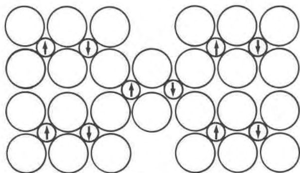
Fig. 1. An idealization of the Cu-O network in dioptase. Arrows in the small circles (Cu) indicate relative spin directions for the proposed magnetic structure. (After Newnham and Santoro, 1967, p. K87).
