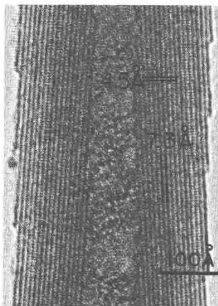
Fig. 9 A typical example of parachrysotile with a weak conical component (Run OS 132).
