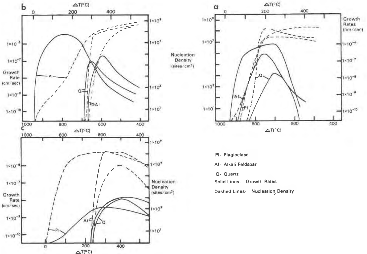
Fig. 5. Combined nucleation density and crystal-growth rate curves. (a) Synthetic granite plus 3.5 wt % H _2 O. (b) Synthetic granodiorite plus 6.5 wt % H _2 O. (c) Synthetic granodiorite plus 12 wt % H _2 O.
