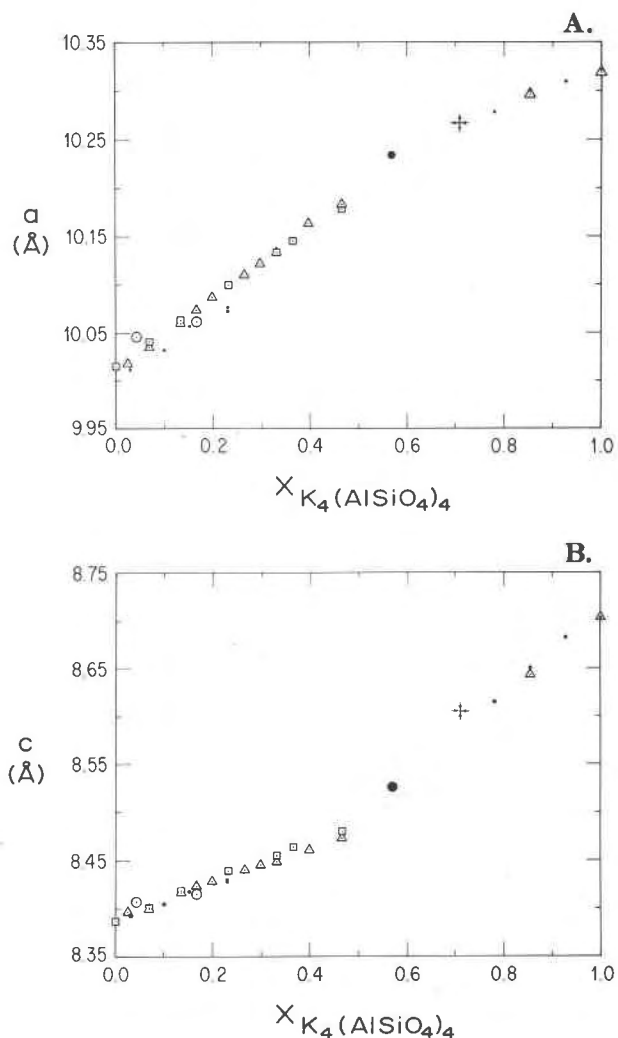
Fig. 1. Unit-cell dimensions (A) a (Fig. 1A) and c (Fig. 1B) for synthetic (\text{Na,K})_3\text{K}(\text{AlSiO}_4)_4 nephelines and kalsilites plotted against mole fraction \text{K}_4(\text{AlSiO}_4)_4 ( X_2 ) in the feldspathoids (the a unit-cell data for kalsilites in Fig. 1A have been multiplied by two). Open circles (Miyashiro and Miyashiro, 1954, Table 2), triangles (Smith and Tuttle, 1957, Tables 2 and 12), and squares (Donnay et al. , 1959, Table IV) represent data for (\text{Na,K})_3\text{K}(\text{AlSiO}_4)_4 nephelines and kalsilites synthesized at one atm in previous investigations. Filled circles depict our data for (\text{Na,K})_3\text{K}(\text{AlSiO}_4)_4 nephelines and kalsilites synthesized at 0.5 kbar, and the radius of each circle indicates the 2\sigma value (A) for the data point (see Table 1). Opposed arrows point to data for the kalsilite synthesized at 0.5 kbar and 904^\circ\text{C} in this study.
