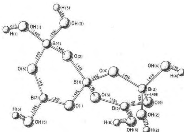
Fig. 4. The borate polyanion [\text{B}_5\text{O}_8(\text{OH})_6]^{9-} and its bond distances.
