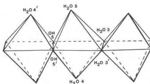
Fig. 2. View of the octahedron of oxygen atoms surrounding Na and the chains formed by edge-sharing. The view is looking down +b^* with +a approximately vertical, +c horizontal to the right ( cf. Table 6).
