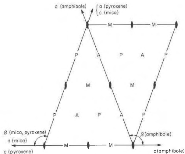
Fig. 4. Section \perp b of a biopyribole unit cell, as in a C2/m mica, a C2/m amphibole, or a C2/c pyroxene. If the amphibole were referred to a body-centered I2/m cell, its axes would correspond to those of a C2/c pyroxene. Mica and pyroxene axes correspond but with a and c reversed. If mica axes were labeled as in pyroxene, it would be A2/m . The 2_1 axes parallel to b are located at points marked M (in mica), A (in amphibole), and P (in pyroxene). 2_1 -axes \parallel b are shown by the standard symbol, and are common to all three.
