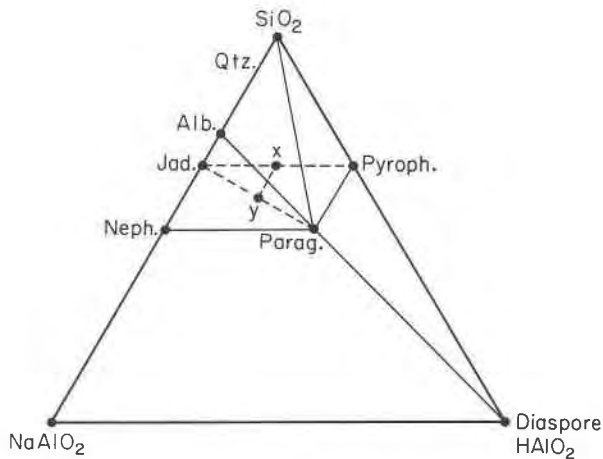
Fig. 9. The composition plane SiO_2-NaAlO_2-HAlO_2 showing the possible dioctahedral amphiboles: Na_2Al_4(Si_8O_{22})(OH)_2-(X) and Na_3Al_4(AlSi_7O_{22})(OH)_2-(Y) , relative to quartz, albite, jadeite, nepheline, paragonite, and pyrophyllite.
