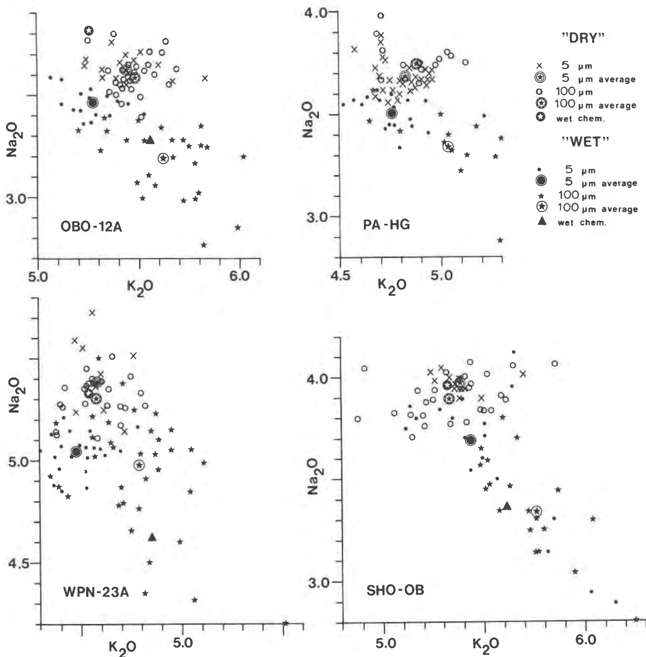
Fig. 1. Analyses of Na 2 O and K 2 O on obsidian and massive perlite in the four samples investigated show typical random scatter of the obsidian analyses around the average, whereas the analyses on perlite define trends of sodium loss and potassium enrichment. These trends, indistinctly outlined by the 5 μm beam analyses, are well defined by the 100 μm beam analyses. The analyses are not recalculated to 100 percent water-free.
