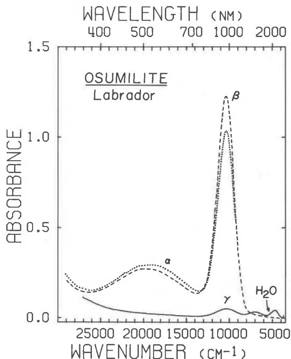
Fig. 4. Room-temperature electronic absorption spectra of an osumilite from Nain. Optic orientation: \gamma = c ; \alpha and \beta occur in the plane normal to the c axis. Crystal thickness = 0.10 mm.
