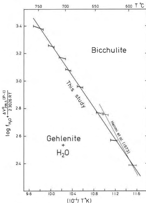
Fig. 3. A log f H 2 O + ΔV 298,8 0 (P - 1)/2.3026 RT vs. 1/T°K plot of the reversal brackets for the reaction bicchulite = gehlenite + H 2 O vapor. Seven heavy brackets are from the present work, the two thin ones are from Henmi et al. (1973).
