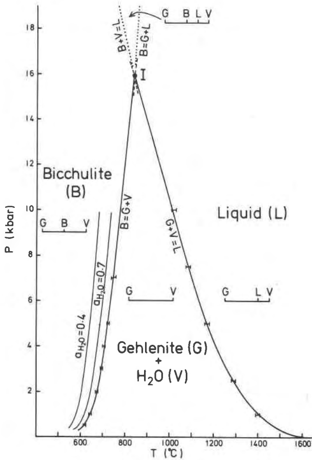
Fig. 4. Phase relations among bicchulite (B), gehlenite (G), a hydrous liquid (L) and H_2O vapor (V) in the system Ca_2Al_2SiO_7-H_2O projected onto the P_{H_2O}(= P_{total}) vs. T °C plane. The equilibrium curves for the decomposition of bicchulite to gehlenite + H_2O vapor at a_{H_2O} equalling 0.7 and 0.4 were calculated from thermodynamic data given in the text.
