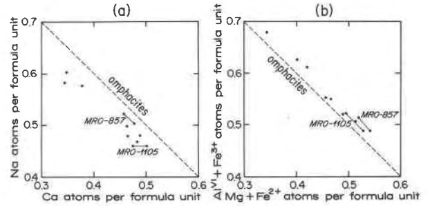
Fig. 5. Proportions of six-coordinated cations per six oxygens in Breuil-St. Jacques clinopyroxenes from eclogites and related rocks from the Zermatt-Saas unit: (a) occupancy of the large M2 site; (b) occupancy of the smaller M1 structural position. Dashed lines indicate the locus of 100 percent filling of the site by the plotted cations; slight but systematic deviations from the lines reflect small proportions of (Mg + Fe^{2+}) residing in M2. Solid lines connect analyses of different grains in samples MRO-857 and MRO-1105. Note that only intermediate (Jd + Ac)-(Di + Hd) compositional ranges are graphed.
