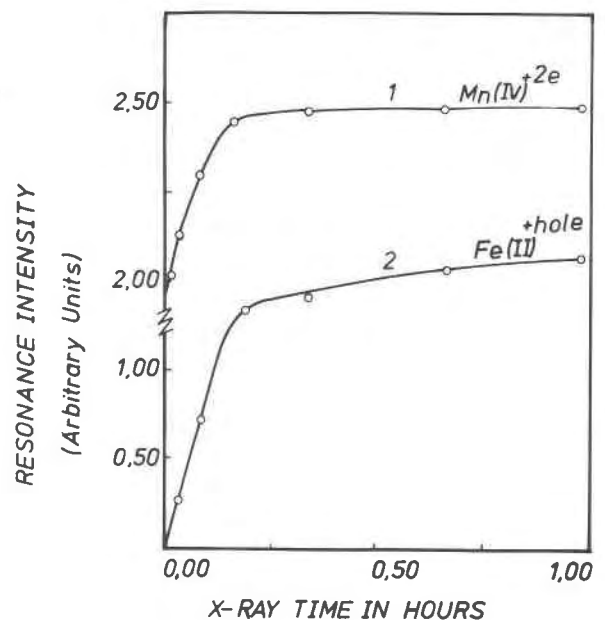
Fig. 4. Growth characteristics of the induced EPR absorption lines with X-ray dosage.
