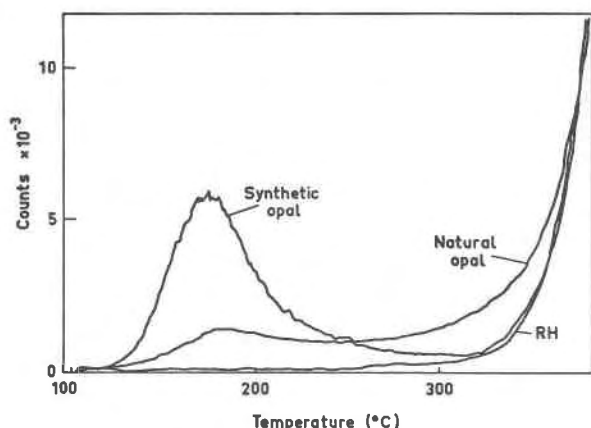
Fig. 6. A comparison of the TL curves from the A Gilson synthetic opal (1) and of the natural Cp2 opal (2) after similar time exposure to fluorescent lighting.
